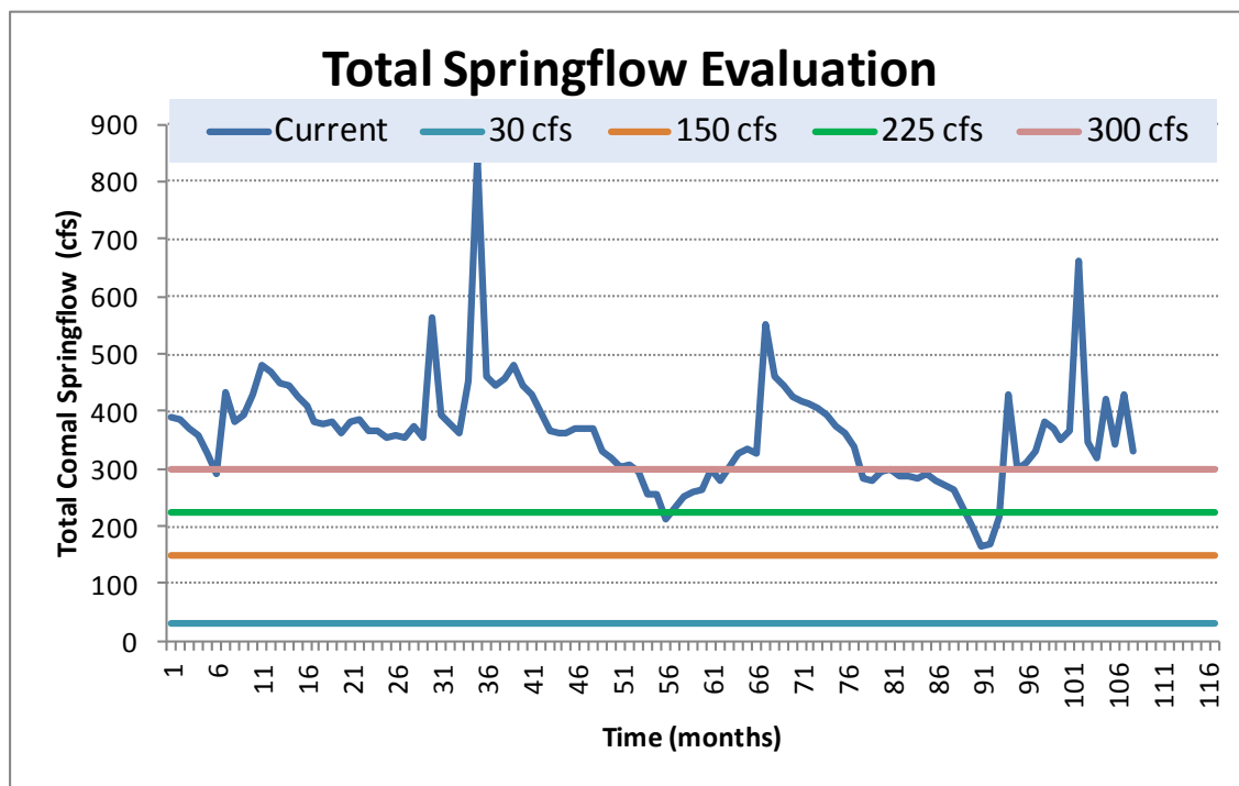
Figure 4-13. Total Comal Springflow scenarios evaluated in Stella. Current pumping is the actual Total Comal Springflow from 2002-2010. Other springflows were held constant.
