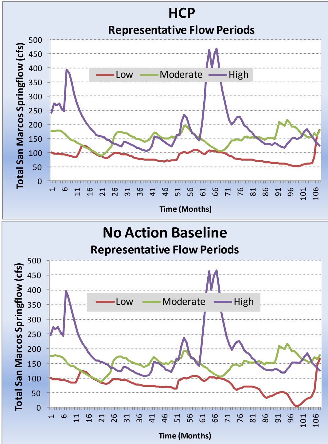
Figure 4-31 and 4-32. Low, Moderate, and High nine-year rolling averages (Total San Marcos springflow) for Phase I package (Top) and No Action baseline (bottom) modeled scenarios.
