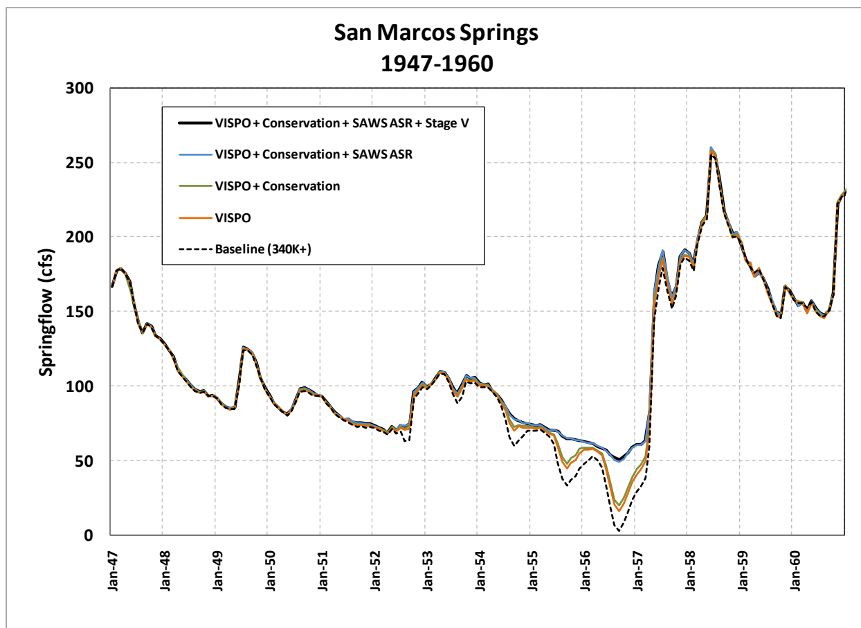
Figure 5-5. Simulated Monthly Average Springflow at San Marcos Springs (1947-1960)
