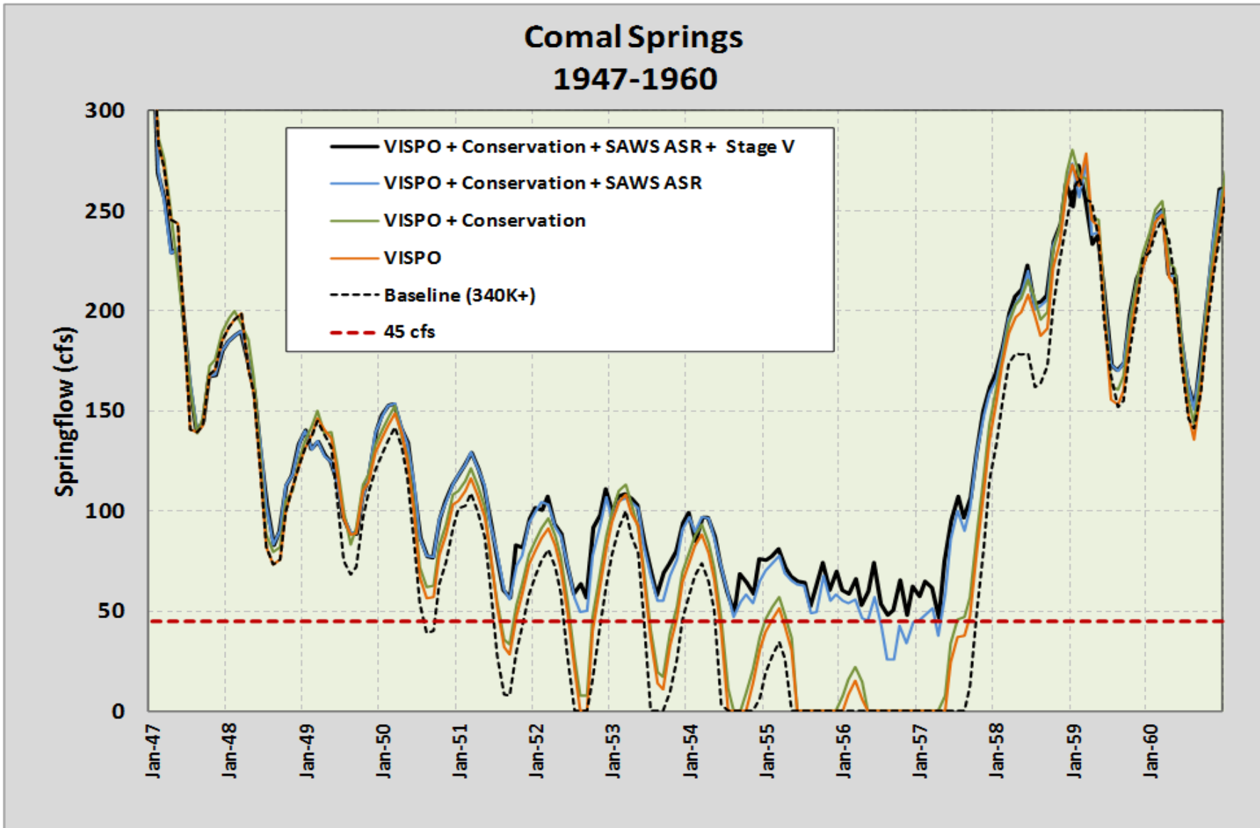
Figure 5-6. Simulated monthly average springflow at Comal Springs (1947-1960) with the specified Phase II Presumptive Measure
