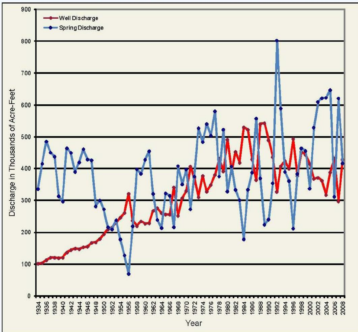
Figure 3-18. Groundwater pumping compared to springflow from the Edwards Aquifer 1934-2009 (EAA 2010a)
