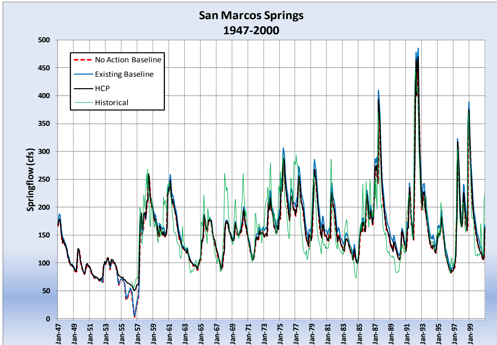
Figure 4-10a. Modeled San Marcos Total Springflow for No Action Baseline, Existing Baseline, and HCP (Phase I) for 1947-2000 model period. (Historical record starts in summer 1956 following gage installation)
