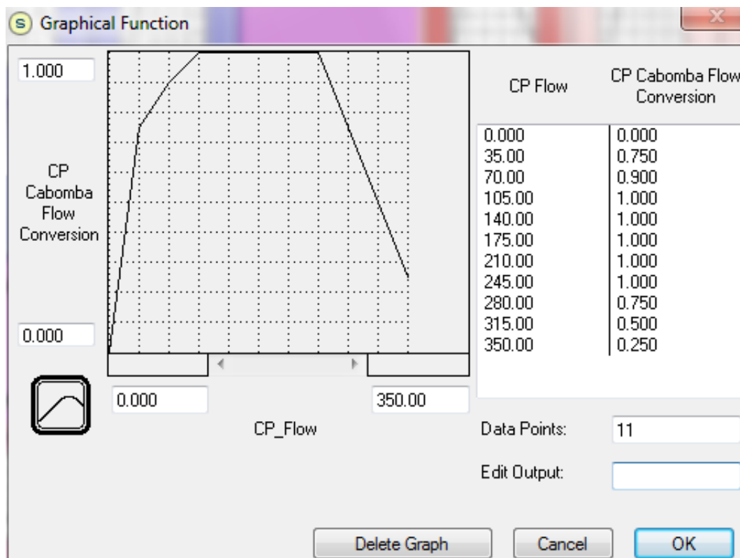
Figure 4-28. Habitat quality relationship for Cabomba versus Total San Marcos springflow, as a daily average, in the City Park reach.
