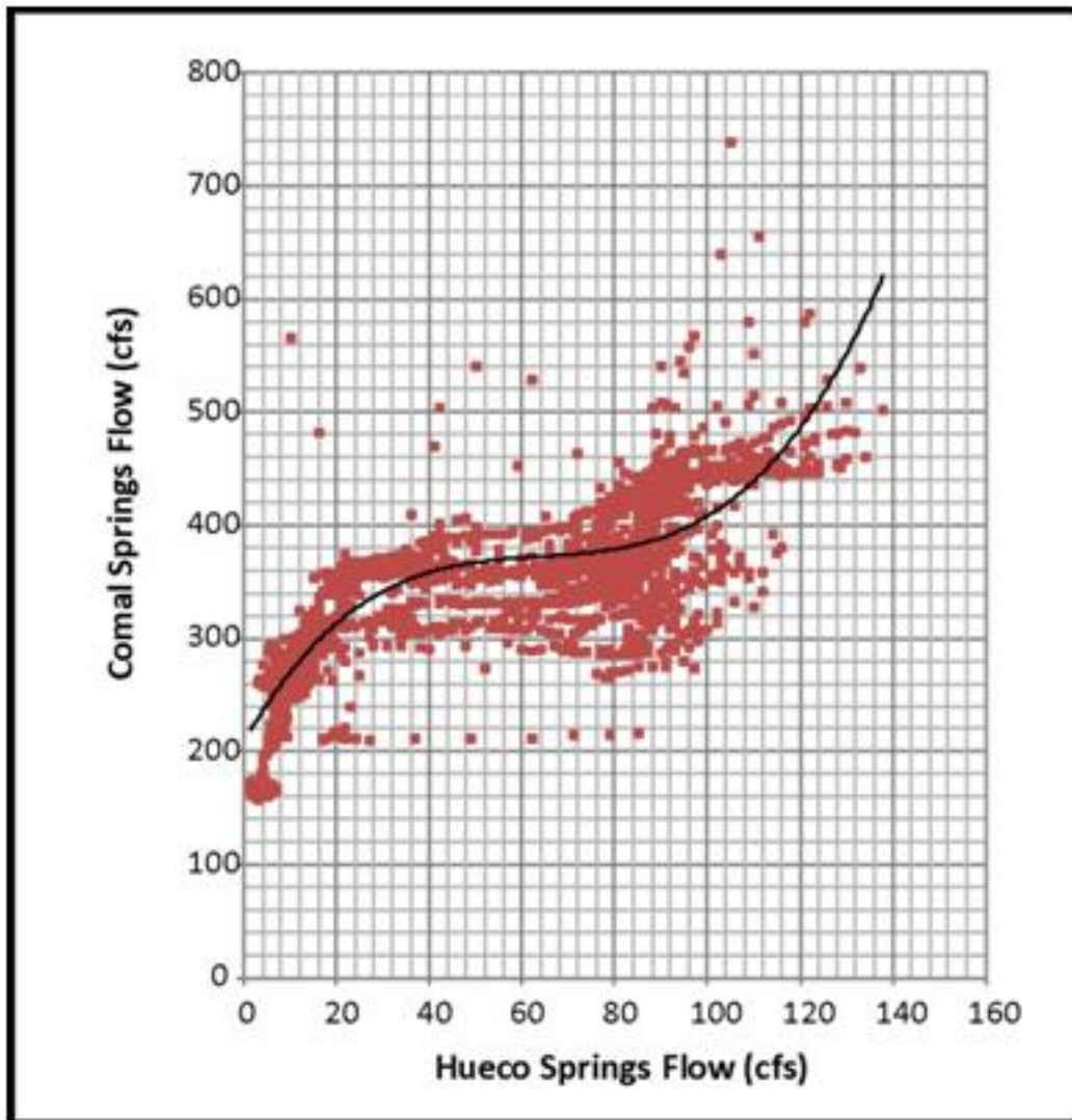
Figure 4-41. Crossplot of Comal and Hueco springflows
