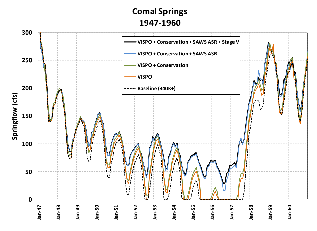
Figure 5-4. Simulated Monthly Average Springflow at Comal Springs (1947-1960)
