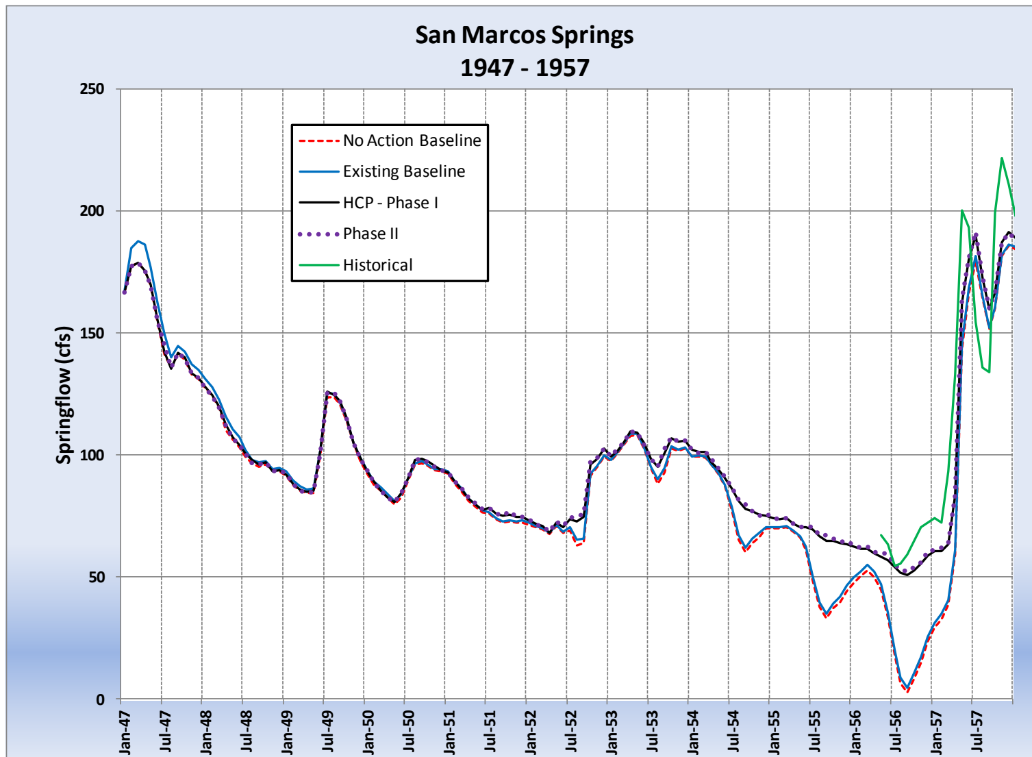
Figure 4-10b. Modeled San Marcos Total Springflow for the No Action Baseline, Existing Baseline, and HCP (Phase I and II) for 1947-1957 model period. (Historical record starts in summer 1956 following gage installation)
