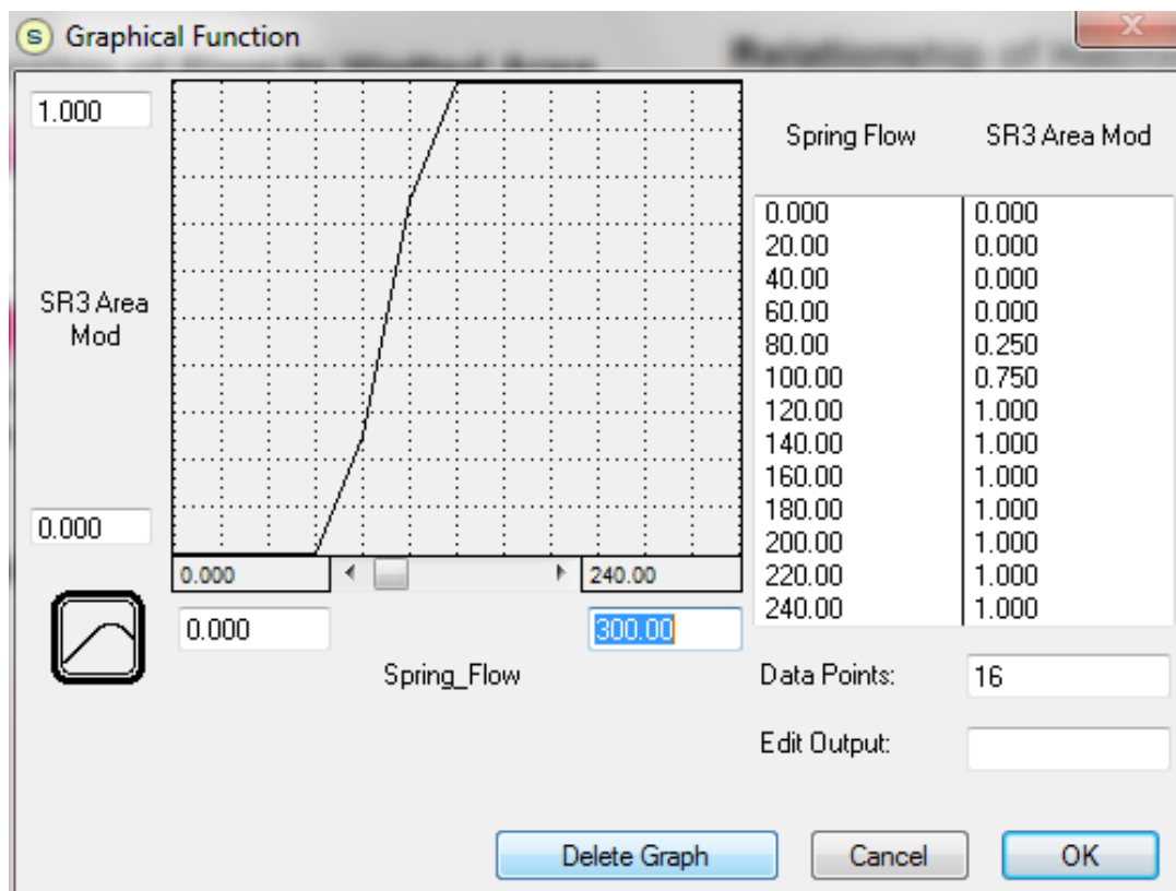
Figure 4-23. Wetted area to flow relationship for Spring Run 3 sample area.
