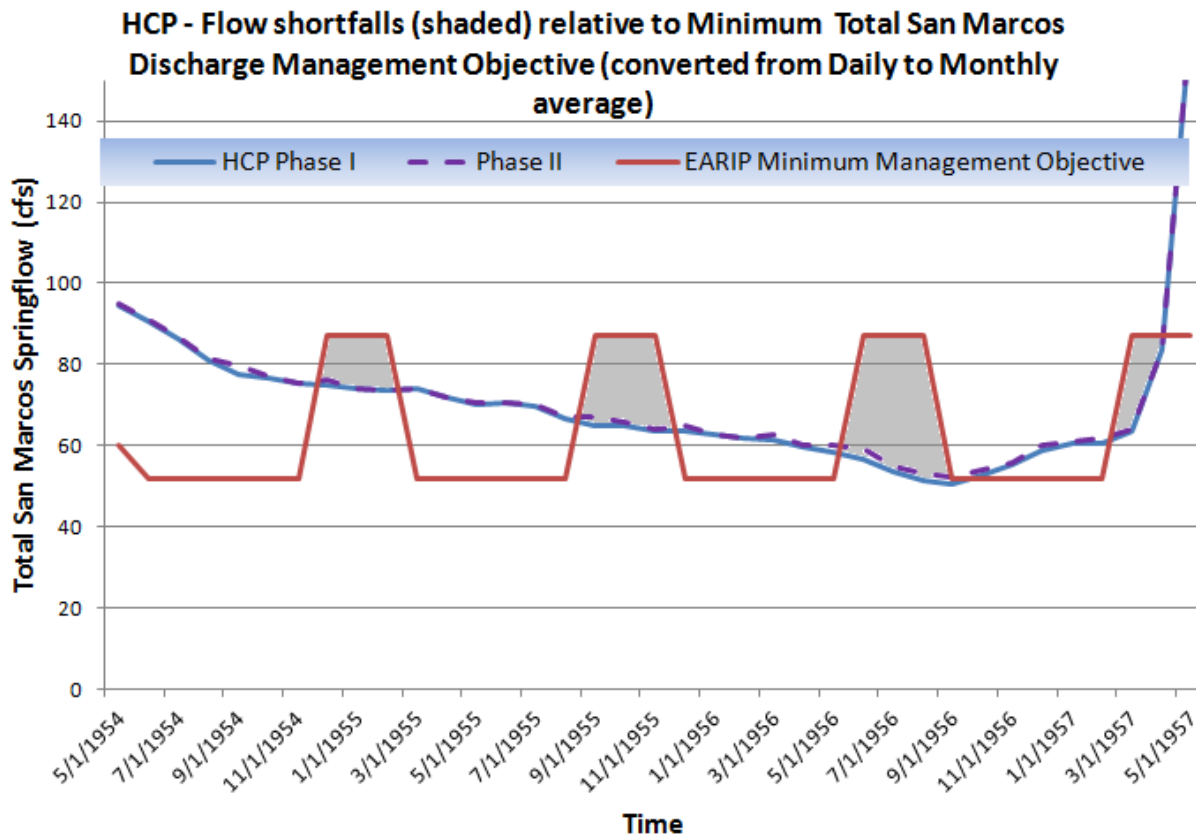
Figure 4-10c. Modeled HCP – Phase I and Phase II San Marcos Total Discharge relative to the higher flows component of the minimum flow objective.
