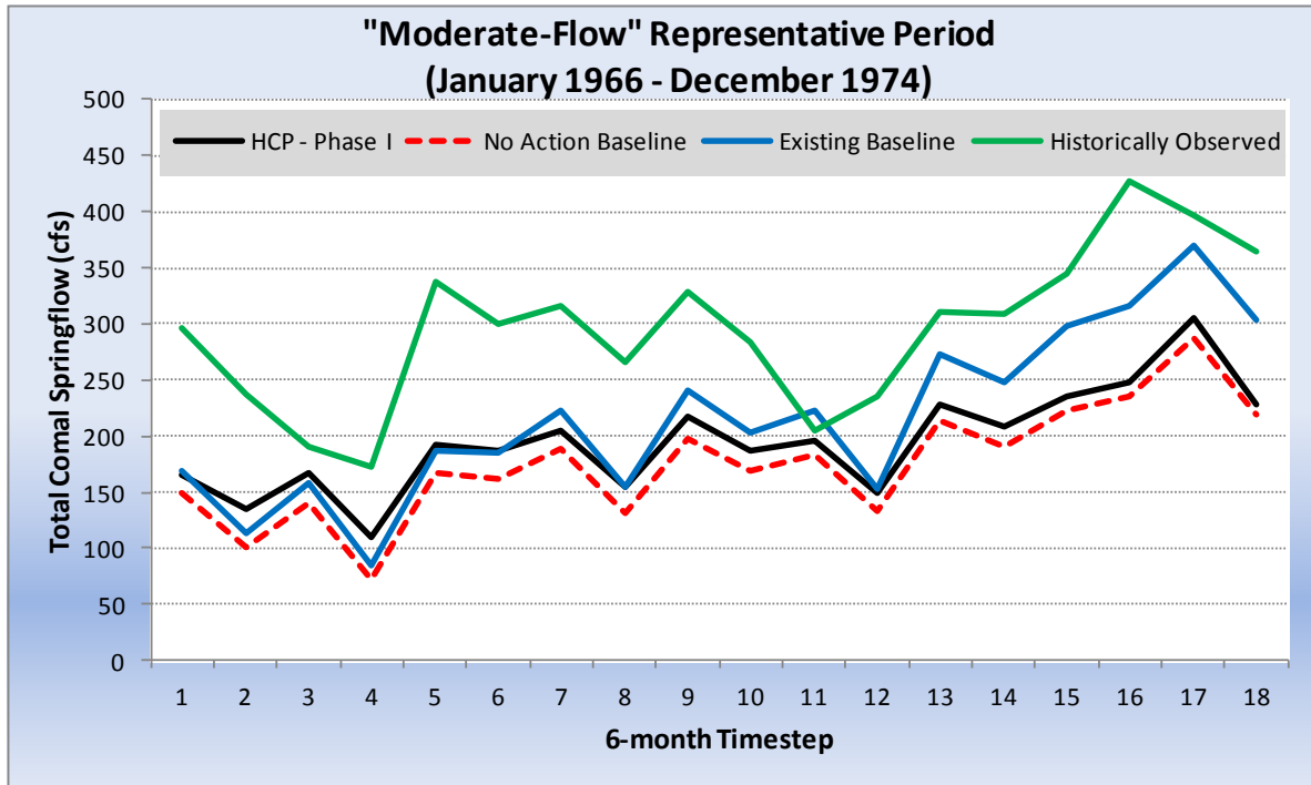
Figure 4-17. Moderate-Flow representative nine-year rolling averages (Total Comal Springflow) for the Phase I package, No Action Baseline, and Existing Baseline modeled scenarios and historically observed.
