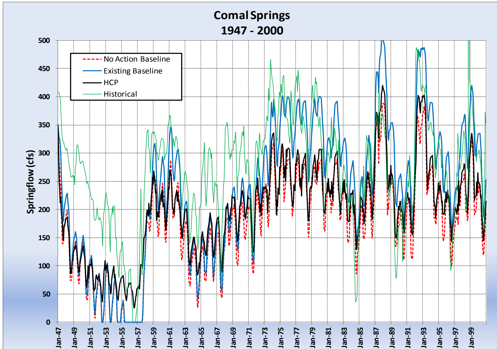
Figure 4-8. Modeled Comal Total Springflow for No Action Baseline, Existing Baseline, and HCP (Phase I) for 1947-2000 model period
