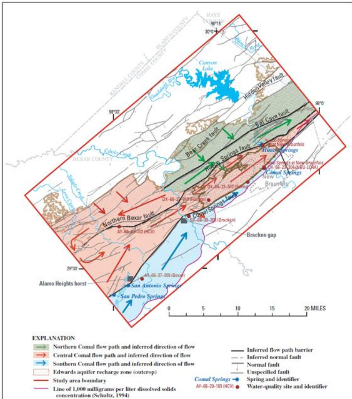
Figure 3-13. Major Faults and Interpreted Groundwater Flowpaths to Comal and Hueco Springs from Otero (2007)
