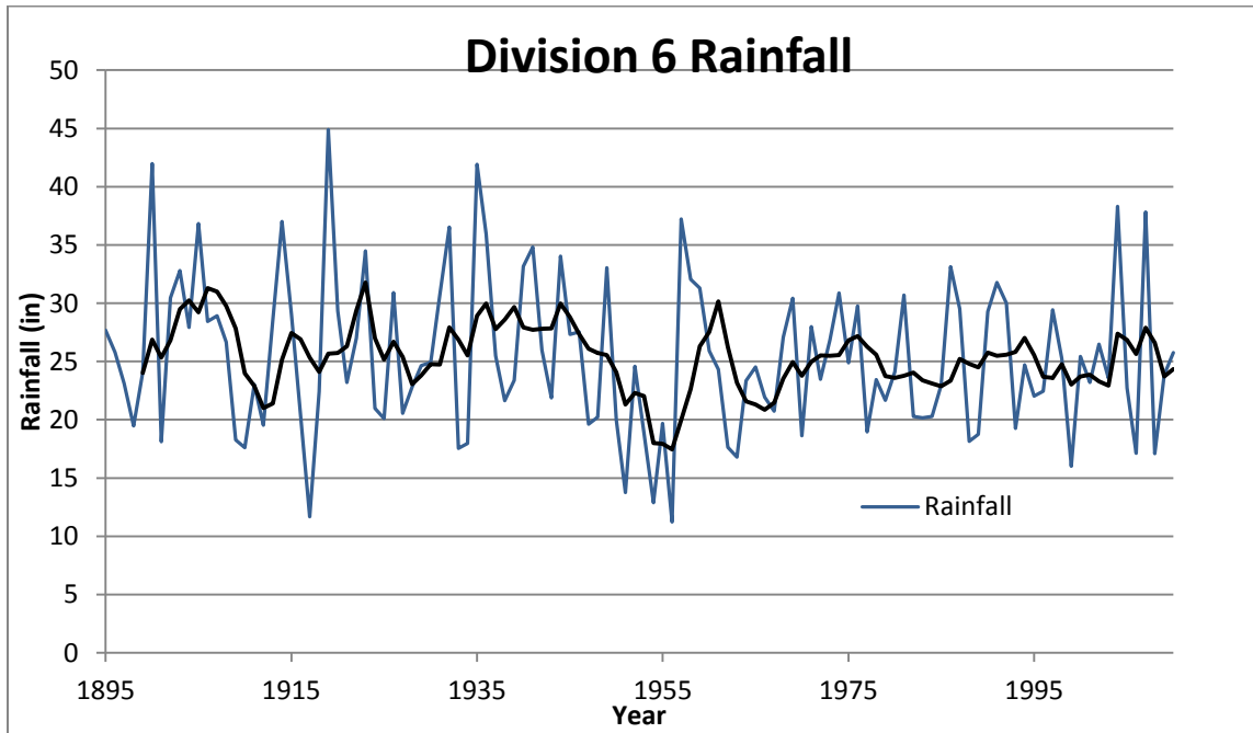
Figure 3-8. Five-year moving average rainfall 1895–2010
