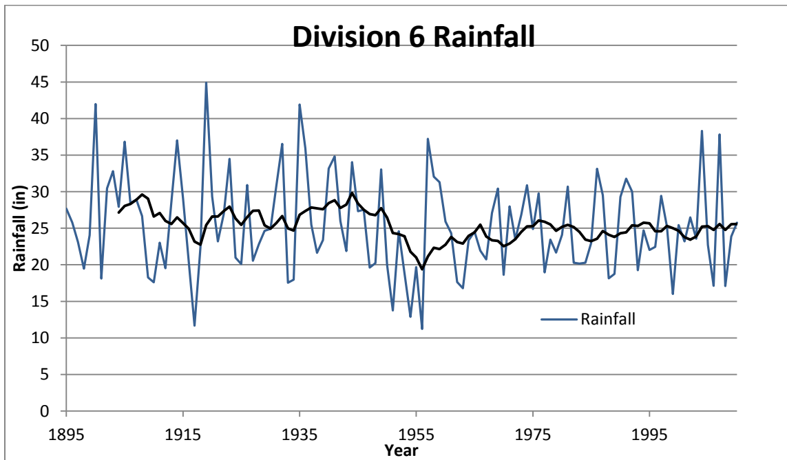
Figure 3-10. Ten-year moving average rainfall 1895–2010
