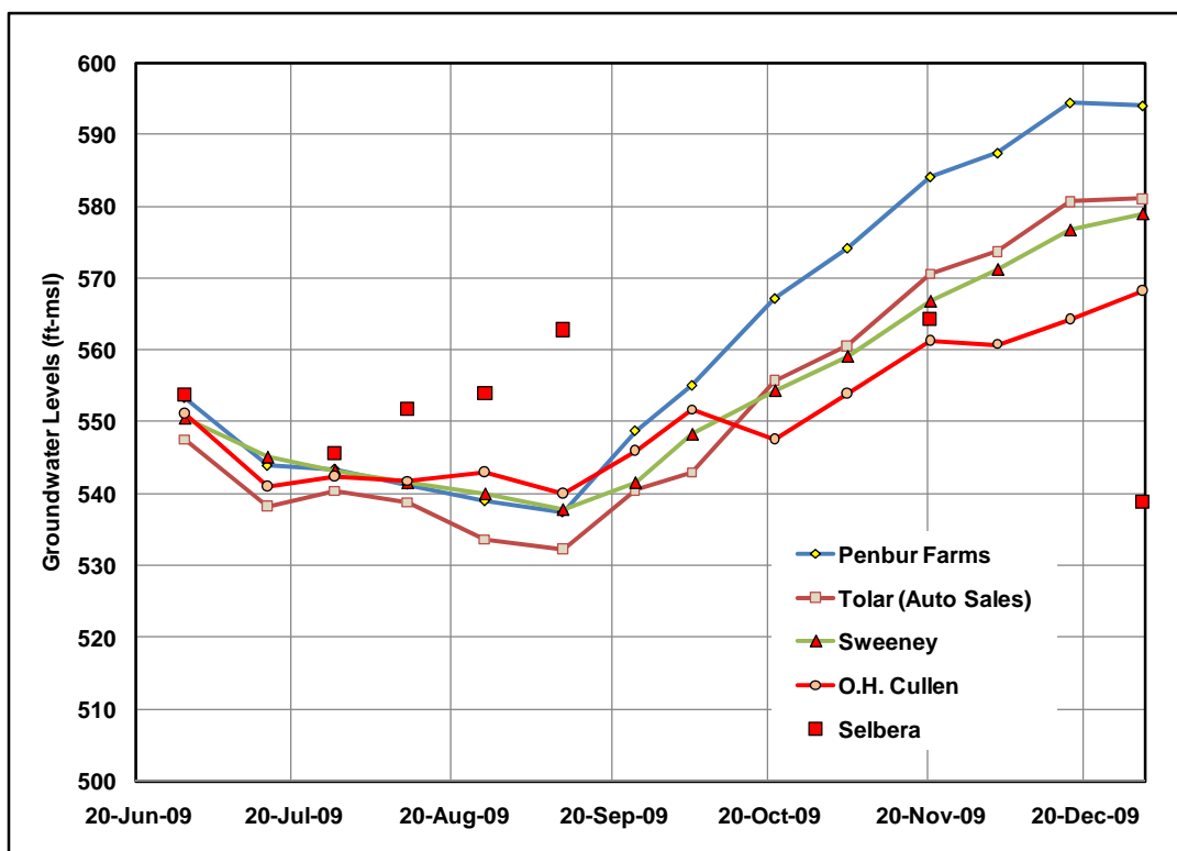
Figure 5-2. Groundwater-Level Hydrographs for 2009 Study Monitor Wells: Kyle to Buda
